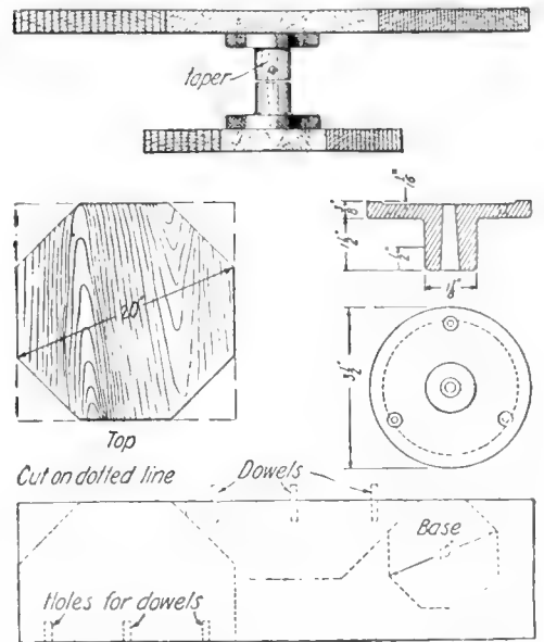
Constructional details of the self-server. The board holding the dishes is mounted on a revolving pin in the center of the table
